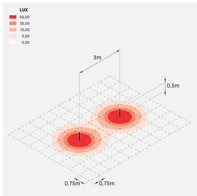
lineDown_post_H500_kit_04
