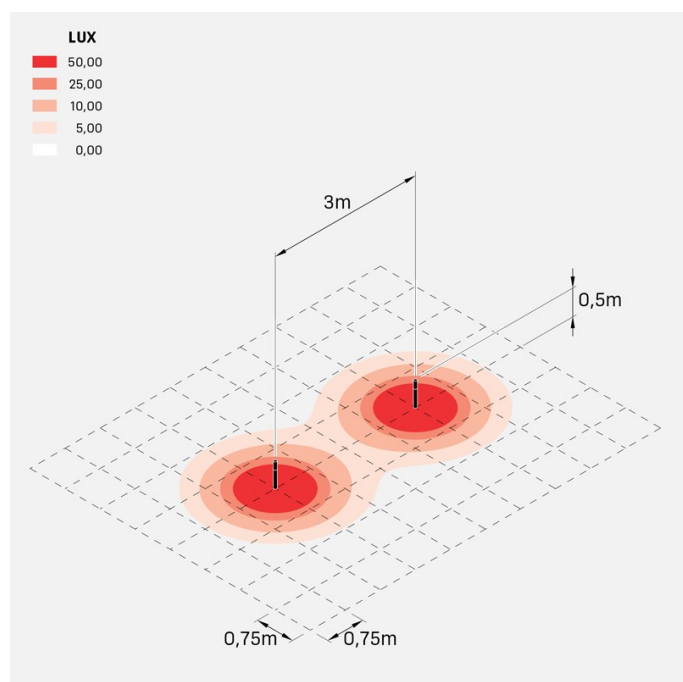
lineDown_post_H500_kit_04
